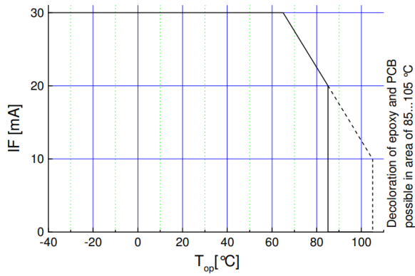
Maximum Ratings (1)
