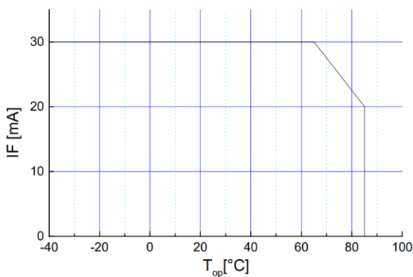
Maximum Ratings (1)
