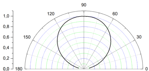
Radiation Pattern
