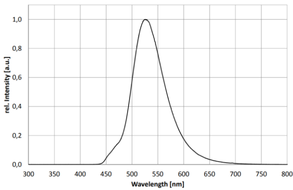
Optical Spectrum
