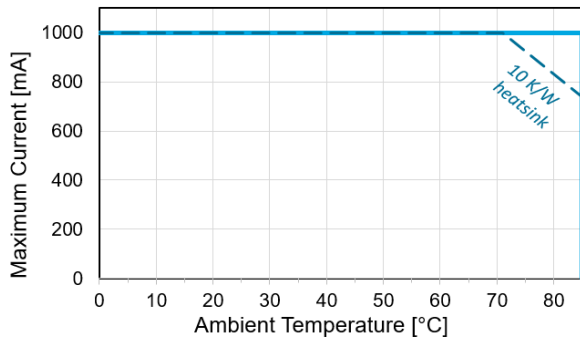
Maximum Ratings (1)
