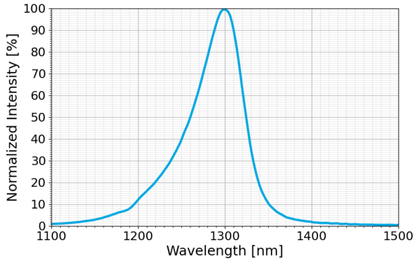
Optical Spectrum
