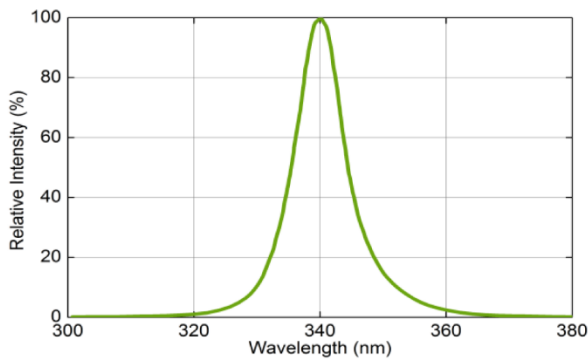
Spectrum @ 350 mA Optical Spectrum
